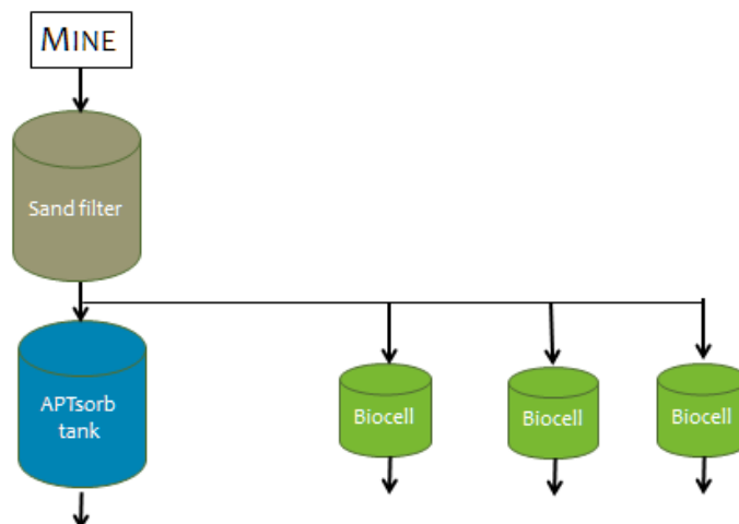
Figure 2: Layout of pilot test, schematic
